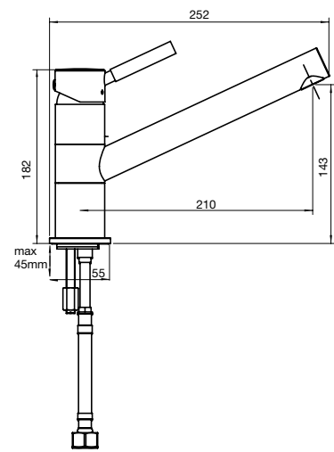
sink mixer
