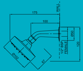
Posh Solus MkII 1 Function Wall Shower on Arm
