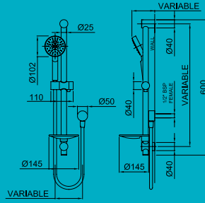
Posh Solus MkII 1 Function Rail Shower
