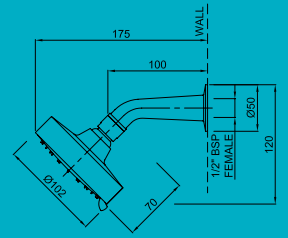
Posh Solus MkII 5 Function Wall Shower on Arm
