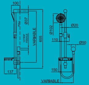
Posh Solus MkII 5 Function Brass Rail Shower
