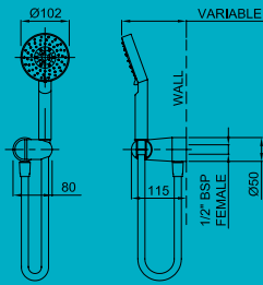
Posh Solus MkII 5 Function Hand Shower
