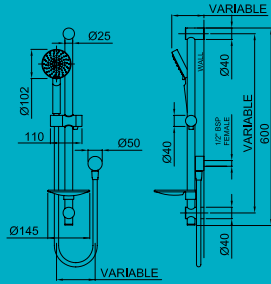
Posh Solus MkII 5 Function Rail Shower
