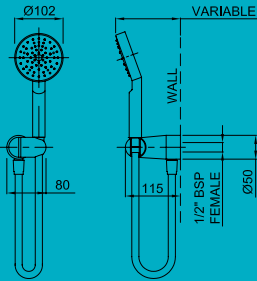
Posh Solus MkII 1 Function Hand Shower
