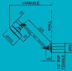
Posh Solus MkII 5 Function Hi-Rise Shower
