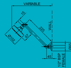
Posh Solus MkII 5 Function Hi-Rise Shower
