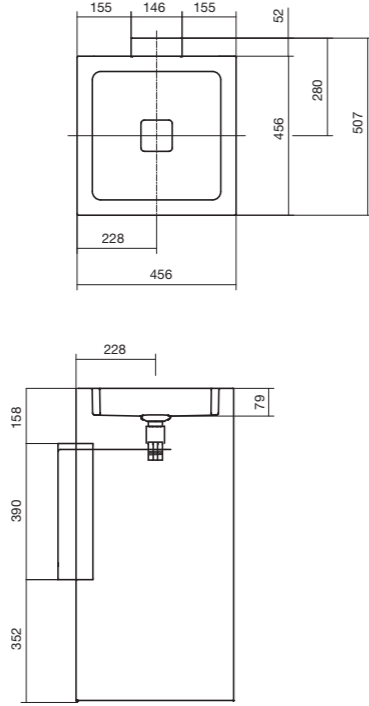
WT 450 Square Freestanding Basin with Square Basin No taphole 9502691
