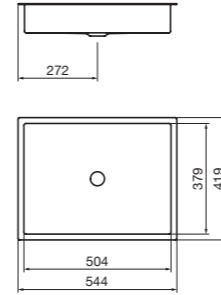
Metaphor 500 Under Counter Basin No taphole 9506282
