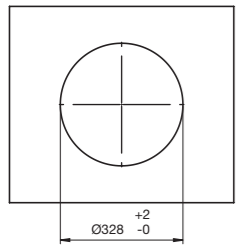
Unisono 325 Semi Inset Basin No taphole 9506195
