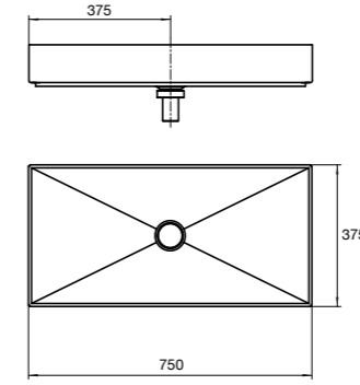
Metaphor 750 Counter Basin No taphole 9502507
