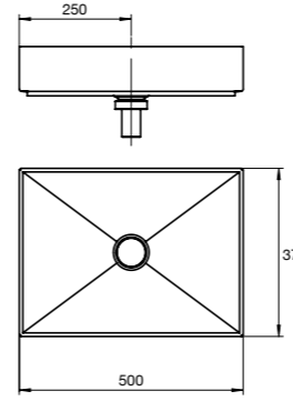
Metaphor 500 Counter Basin No taphole 9502483
