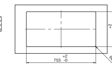
Metaphor 750 Flush Mounted Basin No taphole 9506196
