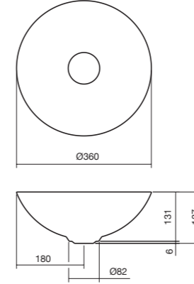
Circa Terra 360 Vessel Basin Gravel Matt 1806078 Nordic Matt 1806079 Oyster Matt 1806080
