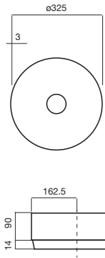
Unisono Counter Basin 325 No taphole 9503961
