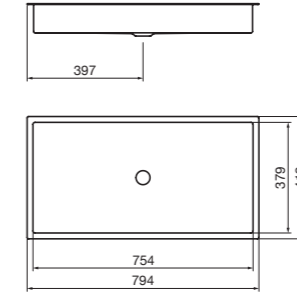
Metaphor 750 Under Counter Basin No taphole 9506283
