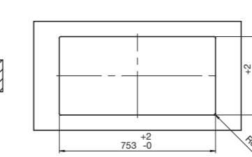
Metaphor 750 Semi Inset Basin No taphole 9506200
