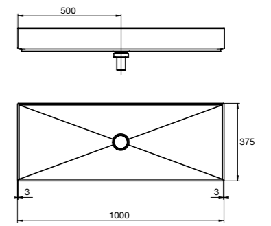
Metaphor 1000 Counter Basin No taphole 9502688
