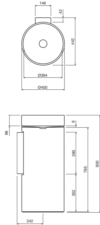
Unisono 400 Freestanding Basin Bi-Colour, No taphole 9508140
