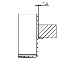
Unisono 325 Semi Inset Basin No taphole 9506195
