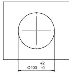
Unisono 400 Semi Inset Basin No taphole 9506193
