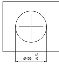
Unisono Counter Basin 400 No taphole 9503959 Also available: Bi-Colour 9508141
