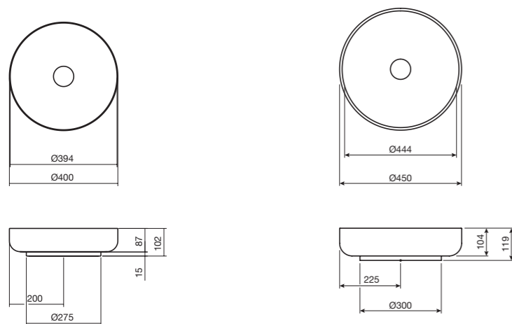
Sondo 400 No taphole 1806081 Also available: Bi-Colour 1806083 Dark Iron 1806082
