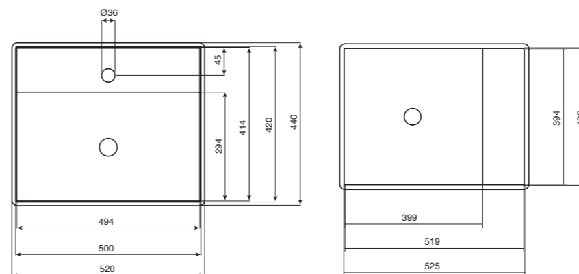
Step 500 Flush Mounted Basin 1 taphole 9506199
