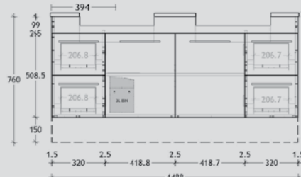
Essence MK II Semi-Recessed 1500mm Double Wall Hung: MER1500WHD With Kick: MER1500WKD
