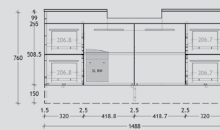
Essence MK II Semi-Recessed 1500mm Single Wall Hung: MER1500WHS With Kick: MER1500WKS
