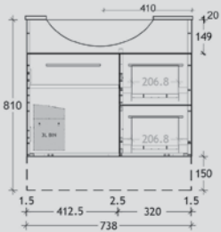
Essence MK II Semi-Recessed 750mm Centre or Offset Wall Hung: MER0750WH With Kick: MER0750WK
