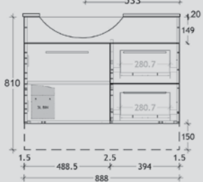
Essence MK II Semi-Recessed 900mm Centre or Offset Wall Hung: MER0900WH With Kick: MER0900WK
