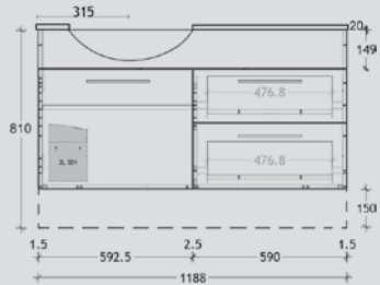
Essence MK II Semi-Recessed 1200mm Offset Wall Hung: MER1200WHO With Kick: MER1200WKO
