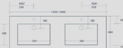
Double
