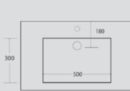
Centre
