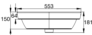
Cygnet Semi Inset Basin 0 Tap Hole
