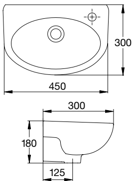
Studio Wall Basin 450
