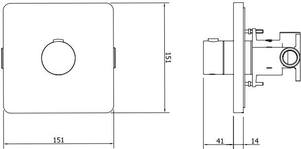
EasySET Thermostatic Mixer
