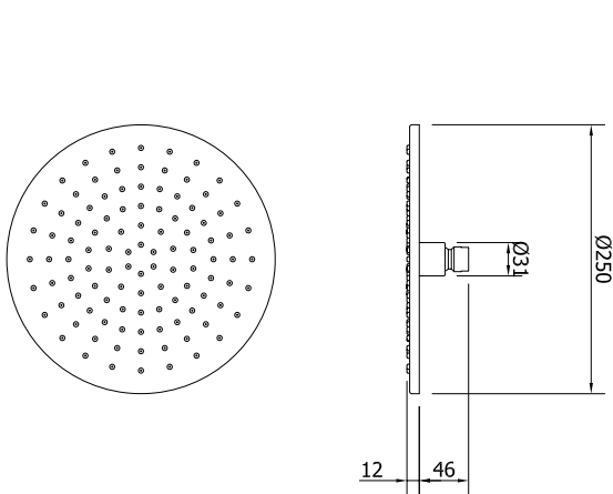
Cygnet Brass Overhead Shower Round
