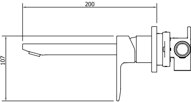
Cygnets Wall Mounted Basin Mixer
