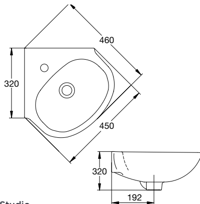
Studio Corner Wall Basin
