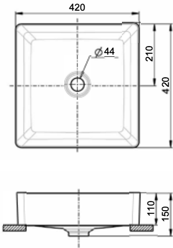
Acacia SupaSleek Square Vessel Basin
