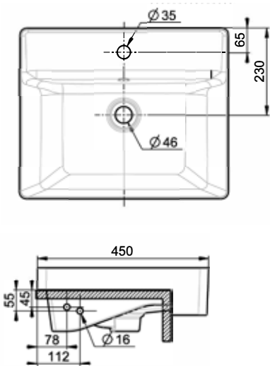
Acacia SupaSleek Semi Recessed Basin
