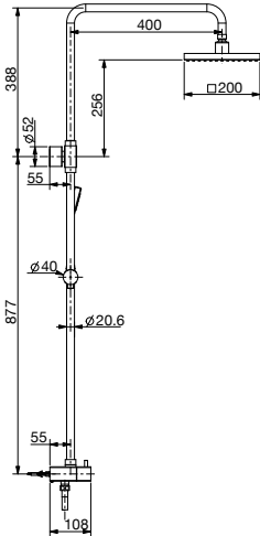
Cygnet Twin Shower Square
