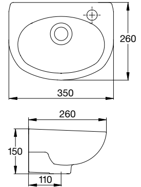
Studio Wall Basin 350
