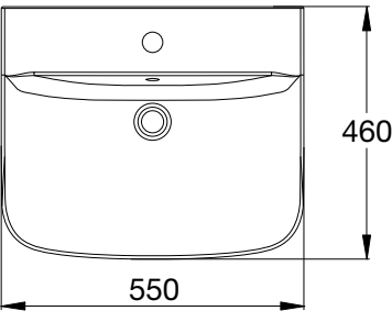
Cygnet Wall Basin
