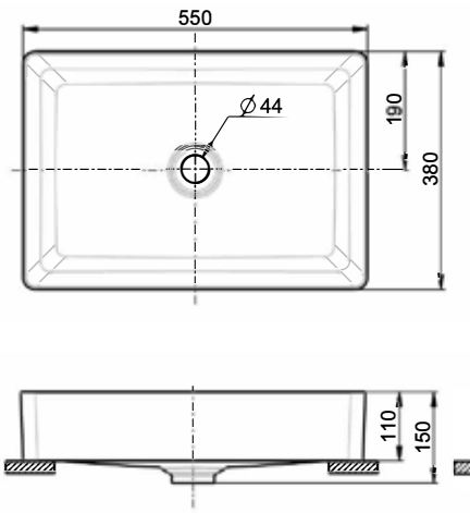
Acacia SupaSleek Vessel Basin
