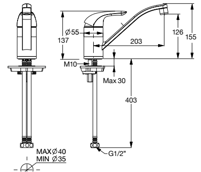
Studio Saga Tubular Sink Mixer
