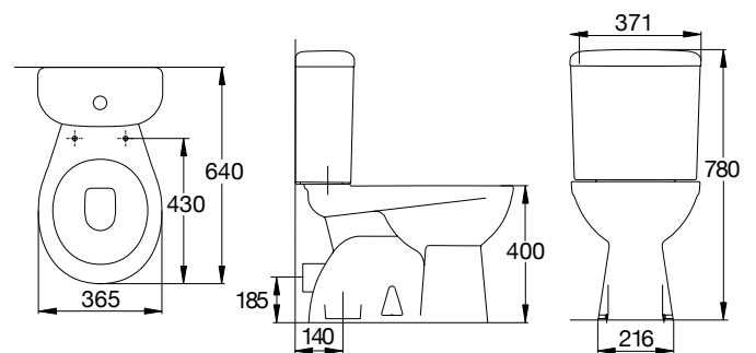
Studio Close Coupled Round Toilet Suite
