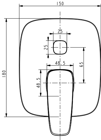
Signature Bath & Shower Mixer with Diverter
