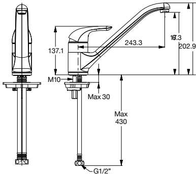
Studio Saga Cast Sink Mixer
