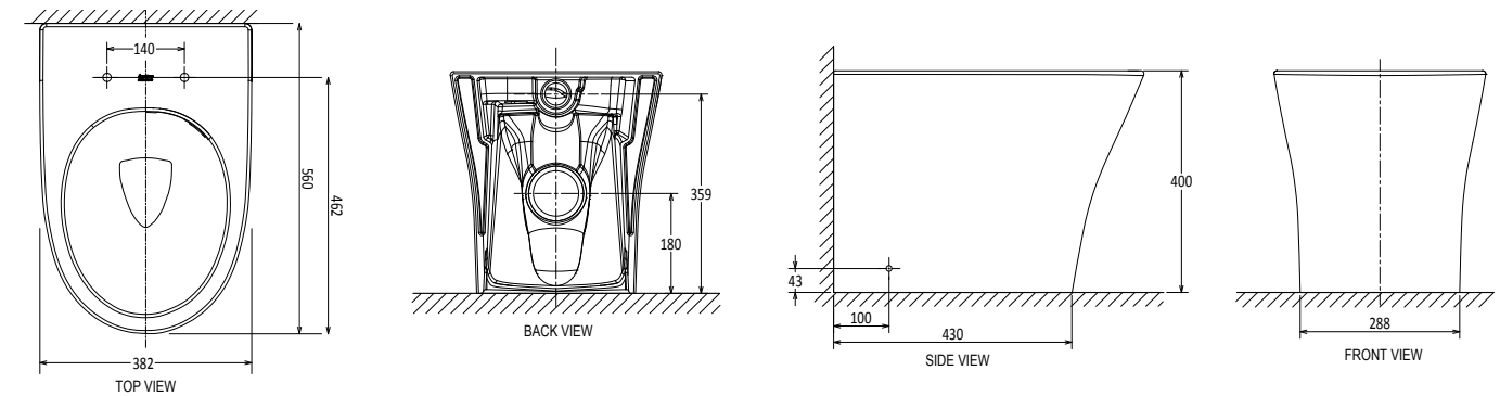
Signature Back to Wall Pan
