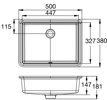
Heron Under Counter Basin
