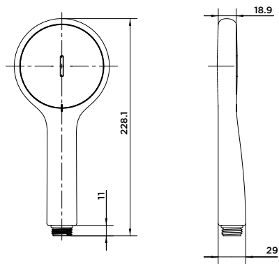
GENIE Hand Shower
