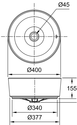
Cygnet Round Vessel Basin
