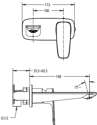
Signature Wall Mount Bath Mixer
