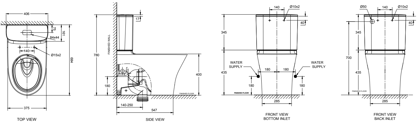
Signature Close Coupled Back to Wall Toilet Suite
