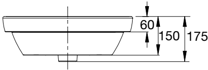
Cygnet Semi Inset Basin 1 or 3 Tap Holes
