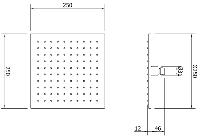
Cygnet Brass Overhead Shower Square
