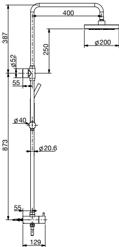
Cygnet Twin Shower Round
