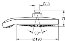
27 765 000 Overhead shower Power and Soul® Cosmopolitan 190
