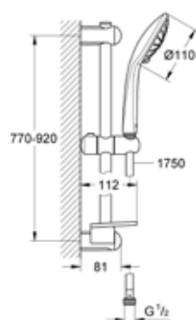
27 226 EN1 27 226 GN0 Rail Shower 110 set
