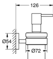
40 448 001 Soap dispenser with holder
