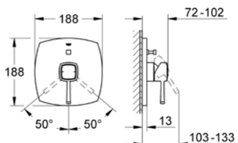
19 920 000 Shower/bath mixer with diverter
