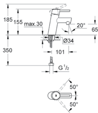
32 253 001 Basin mixer
