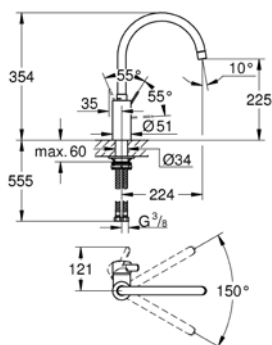
31 188 002 Eurosmart Cosmopolitan
