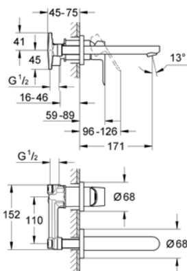
29 220 000 Wall mounted basin mixer set
