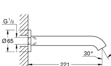
133 392 001 Wall mounted bath spout
