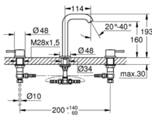
20 596 001 Basin set with separate concealed body
