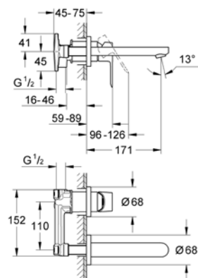
29 219 000 Wall mounted bath mixer set
