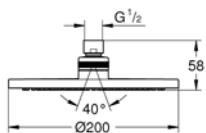
26 497 001 Overhead shower 200
