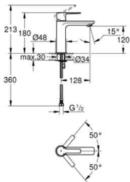
32 252 001 Basin mixer
