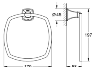
40 630 000 Towel ring
