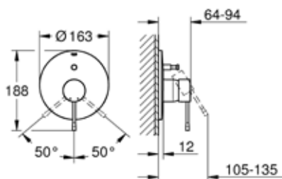
30 270 EN0 30 270 A00 30 270 GN0 Shower/ bath mixer with diverter
