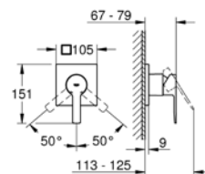
29 169 001 Shower/bath mixer
