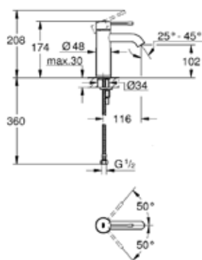
23 860 EN1 23 860 A01 23 860 GN1 Essence Basin Mixer
