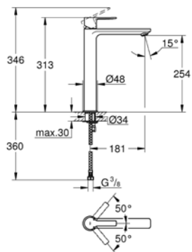
23 861 001 Extended basin mixer
