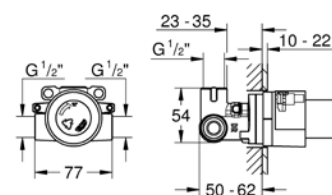
32 962 001 Single-lever mixer 1/2" concealed body
