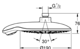
27 767 000 Overhead shower Power and Soul® 190
