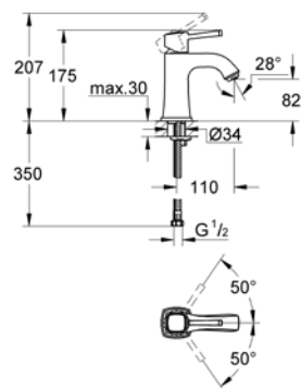
23 321 000 Basin mixer
