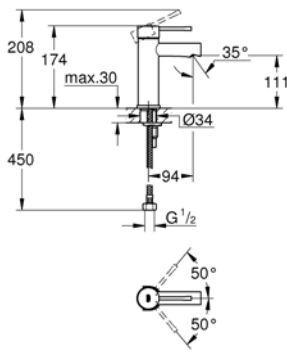
32 215 001 Basin mixer
