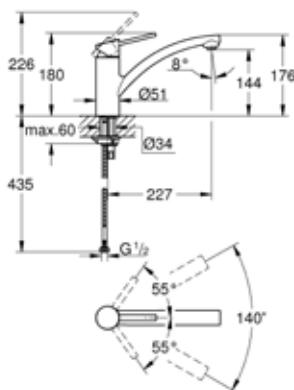
30 363 000 Swift sink mixer
