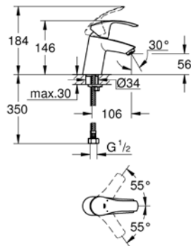
33 161 002 Basin mixer
