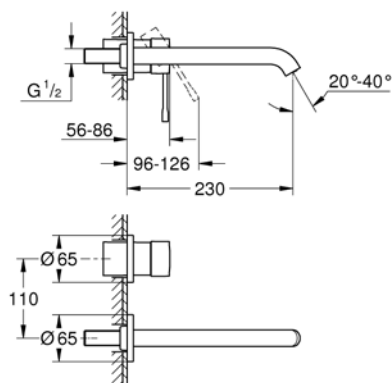
19 967 EN1 19 967 A01 19 967 GN1 Wall mounted basin mixer set
