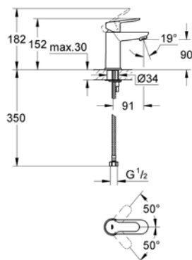
23 176 000 Basin mixer
