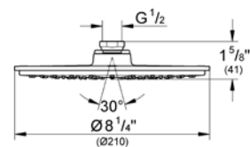
28 373 000 Overhead shower Rainshower® 210
