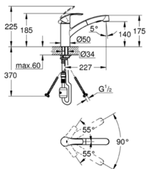
30 317 000 Eurosmart New sink mixer with pull-out spray
