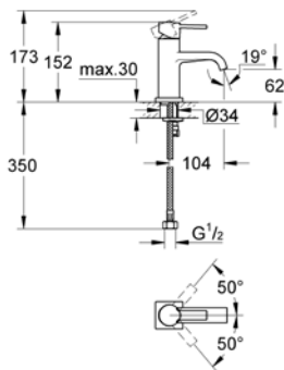
32 759 000 Basin mixer
