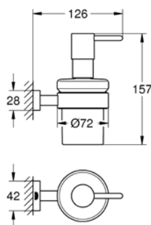
40 756 001 Soap dispenser with holder
