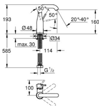
23 488 EN1 23 488 A01 23 488 GN1 Basin Mixer
