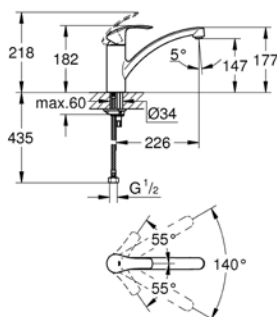
32 534 002 Eurosmart New sink mixer
