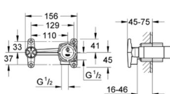
23 319 000 Single-lever mixer 1/2" concealed body
