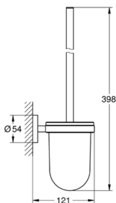
40 374 001 Toilet brush set
