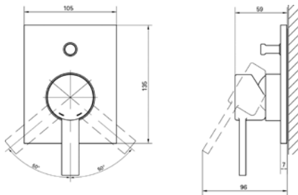
19 315 000 Shower/bath mixer with diverter (Exclusive in ANZ*)
