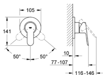
19 587 000 Shower/bath mixer
