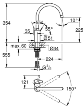
31 188 002 Sink mixer C-spout
