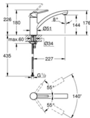
30 363 000 Sink Mixer low spout
