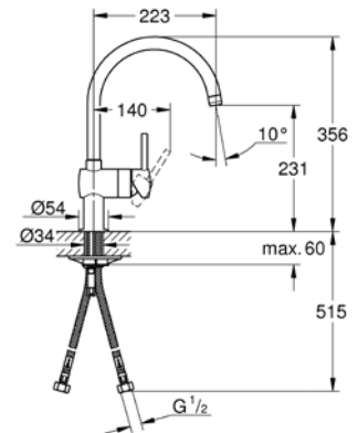
32 930 000 Sink mixer C-spout
