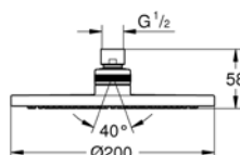
26 497 001 Overhead shower Tempesta 200
