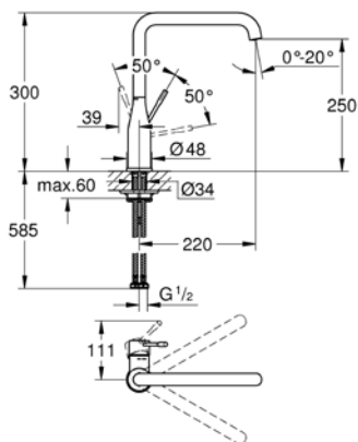
30 372 000 Sink Mixer
