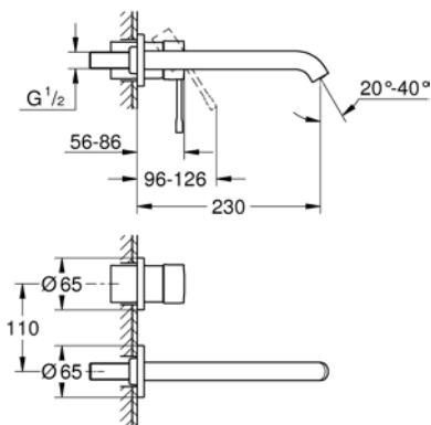
19 967 001** Wall mounted basin mixer set 230mm
