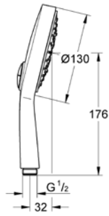
26 525 000 Hand shower Power&Soul® Cosmopolitan 130
