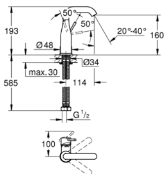
23 488 EN1 23 488 A01 23 488 GN1 Basin Mixer
