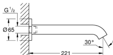
13 392 EN1 13 392 A01 13 392 GN1 Essence bath spout
