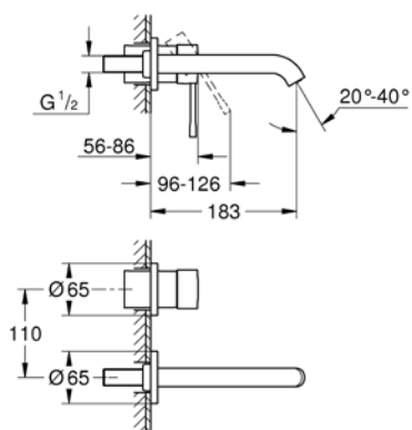
19 408 EN1 19 408 A01 19 408 GN1 Wall mounted basin mixer set
