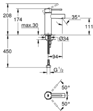
32 215 001 Basin mixer
