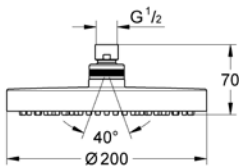
27 541 000 Overhead shower New Tempesta Cosmopolitan 200
