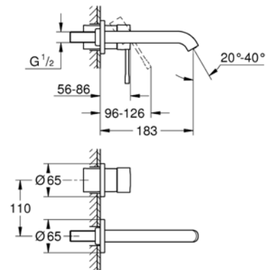
29 134 001 Wall mounted basin mixer set 183mm
