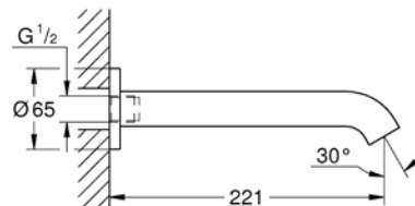
133 392 001 Wall mounted bath spout Projection 220mm
