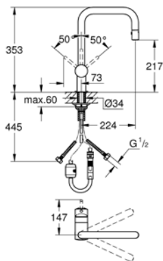
31 116 000 Sink mixer U-spout with pull-out spray
