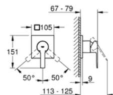
29 169 001 Shower/bath mixer
