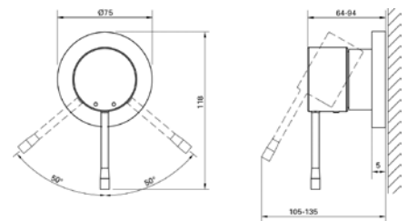
29 258 001 Shower/bath mixer (Exclusive in ANZ*)
