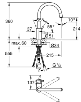
31 117 003 Sink mixer with pull-out spray
