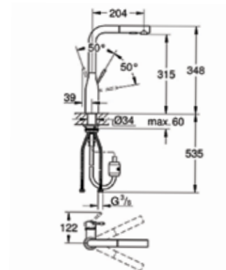
30 371 EN0 30 371 A00 30 371 GN0 Sink Mixer high spout
