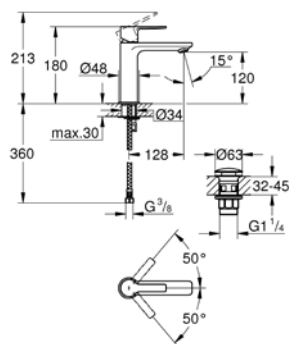
32 252 001 Basin mixer
