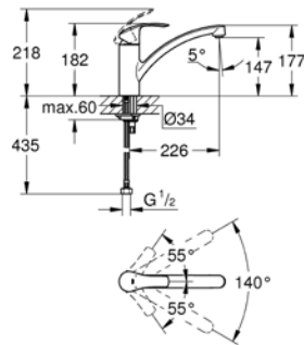
32 534 002 Sink mixer low spout
