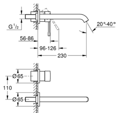
19 967 EN1 19 967 A01 19 967 GN1 Wall mounted basin mixer set
