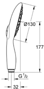
26 527 000 Hand shower Power&Soul® 130
