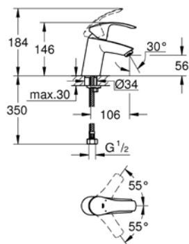
33 161 002 Basin mixer
