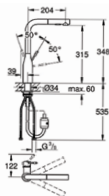
30 371 000 Sink mixer high spout with pull-out dual spray
