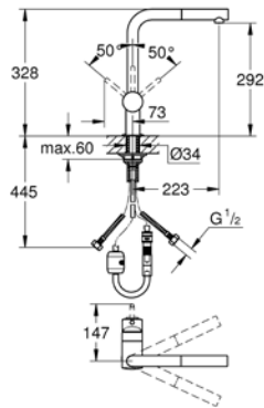
31 115 000 Sink mixer L-spout with pull-out spray
