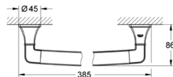
40 633 000 Grab rail
