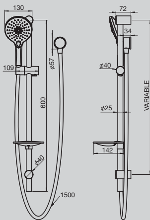
Domaine 3 Function Rail Shower
