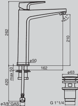
Solus MK2 Extended Basin Mixer
