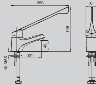
Bristol MK2 Basin Mixer with Extended Lever Handle
