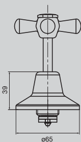
Bristol Wall Top Assembly
