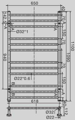
Domaine Heated Towel Rail 1100mm h x 650mm w
