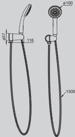
Solus MK2I 1 Function Hand Shower
