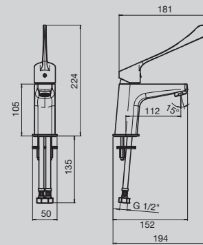
Solus MK3 Extended Lever Basin Mixer
