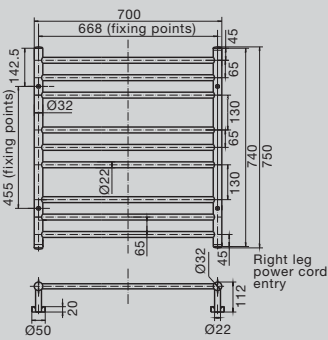
Domaine Heated Towel Rail 750mm h x 700mm w
