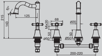
Canterbury English Basin Set
