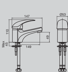
Bristol MK2 Basin Mixer
