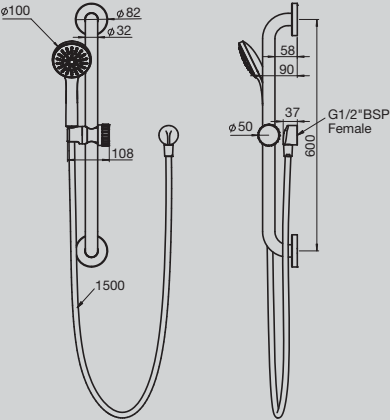
Solus MK2I 1 Function 600mm Grab Rail Shower
