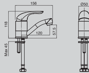
Bristol MK2 Swivel Basin Mixer
