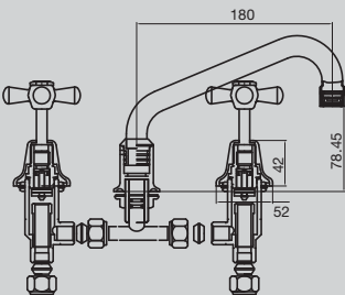
Bristol Hob Sink Set
