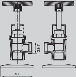
Solus Washing Machine Stops
