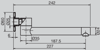
Solus MK2 Swivel Bath Outlet
