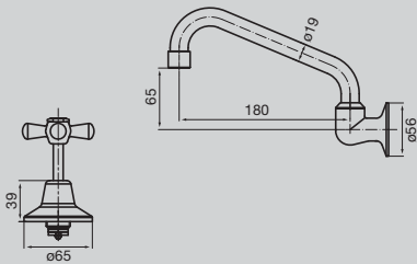
Bristol Wall Sink Set
