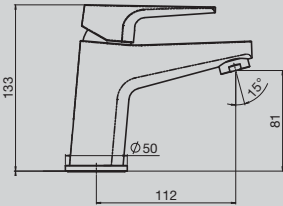
Solus MK2 Basin Mixer
