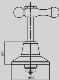
Bristol Wall Top Assembly Lever Handle
