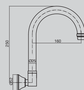
Bristol Gooseneck Wall Outlet
