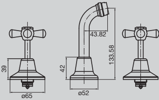
Bristol Wall Bath Set
