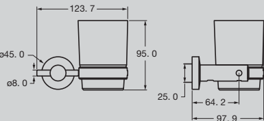
Solus MK2 Single Tumbler
