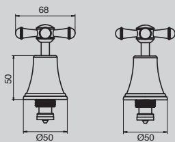
Canterbury Wall Top Assemblies
