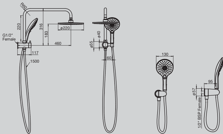
Domaine Short Twin Rail Shower
