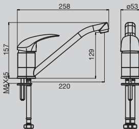
Bristol MK2 Sink Mixer
