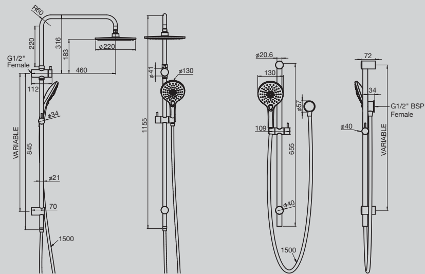
Domaine Twin Rail Shower
