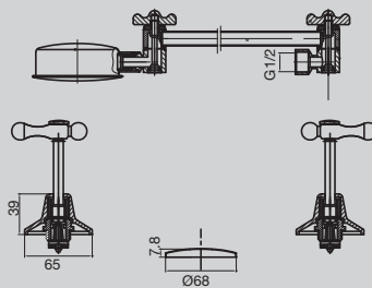
Bristol Shower Set Lever Handle
