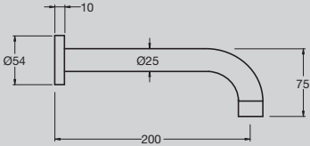
Solus Curved Bath Outlet
