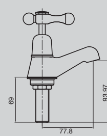
Bristol Pillar Taps Lever Handle
