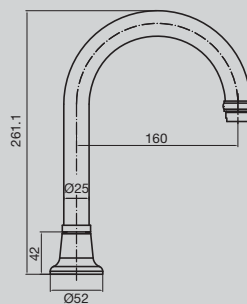
Bristol Gooseneck Hob Outlet 25mm
