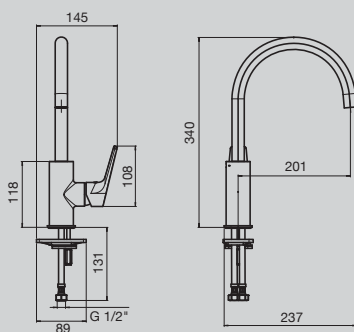
Solus MK3 Gooseneck Sink Mixer
