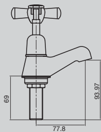
Bristol Pillar Taps
