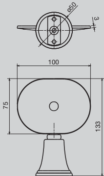
Canterbury Double Towel Rail 300mm / 750mm / 900mm
