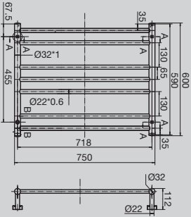
Domaine Heated Towel Rail 600mm h x 750mm w
