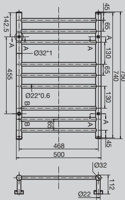
Domaine Heated Towel Rail 750mm h x 500mm w
