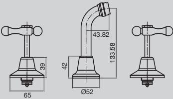
Bristol Wall Bath Set Lever Handle
