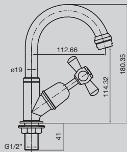
Bristol Rainwater Tap
