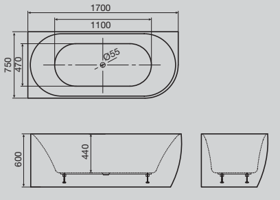
Solus 1700 Back to Corner Freestanding Bath
