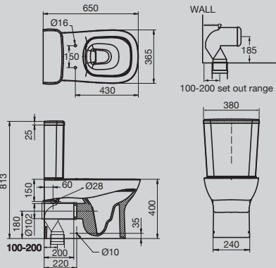
Domaine Close Coupled Back to Wall Rimless Toilet Suite Back Inlet
