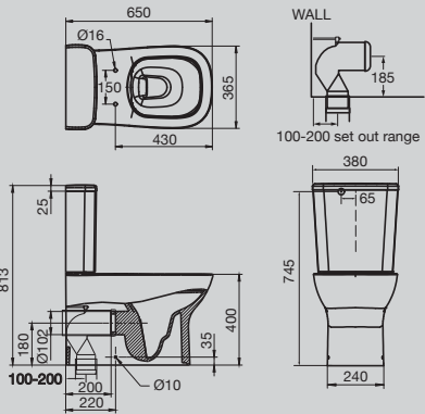
Domaine Close Coupled Back to Wall Rimless Toilet Suite Bottom Inlet
