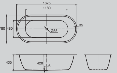
Solus Oval Inset Bath
