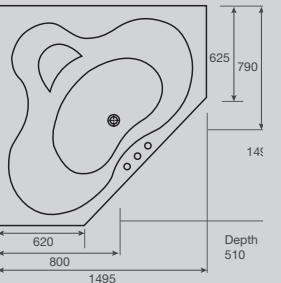
Solus MK2 Corner Santai Spa
