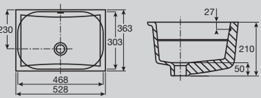
Solus Under Counter Basin 530 x 365mm
