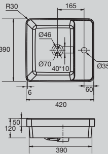
Domaine Semi Inset Basin
