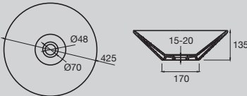
Solus Vessel Basin 425mm
