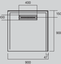
Solus MK2 Shower Base
