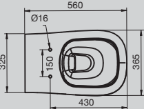
Domaine Close Coupled Back to Wall Rimless Toilet Suite Back Inlet
