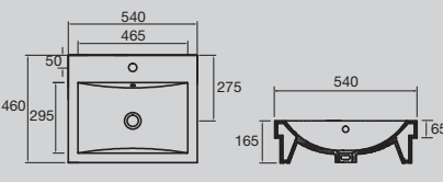
Solus Semi Inset Basin 540 x 460mm
