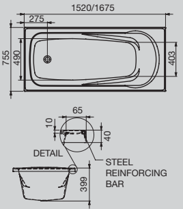
Solus MK2 Rectangular Inset Bath
