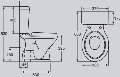
Solus Square Close Coupled S Trap Toilet Suite
