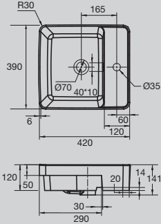
Domaine Semi Recessed Basin
