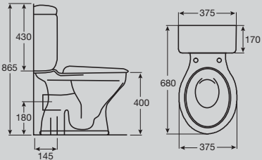
Solus Round Close Coupled S Trap Toilet Suite
