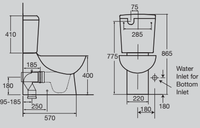
Solus Square Close Coupled Back to Wall Toilet Suite
