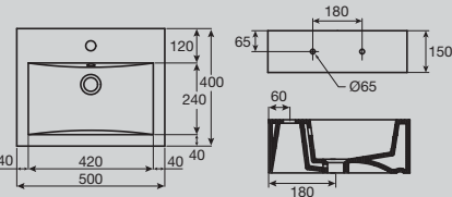
Solus Wall Basin 500 x 400mm
