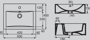
Solus Counter Basin
