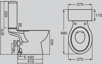
Solus Round Close Coupled P Trap Toilet Suite
