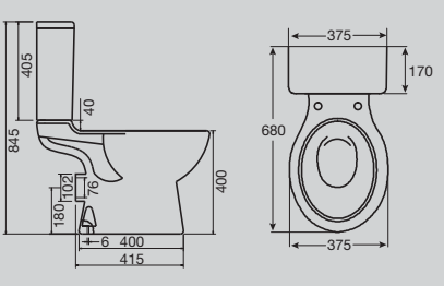
Solus Square Close Coupled P Trap Toilet Suite
