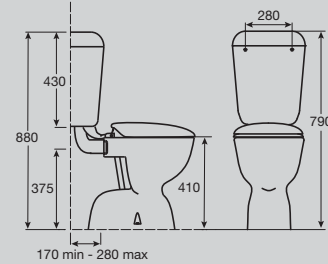
Solus Round Link Toilet Suite
