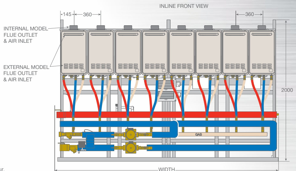
Inline 7 -12 Commpak Plus® Front view
